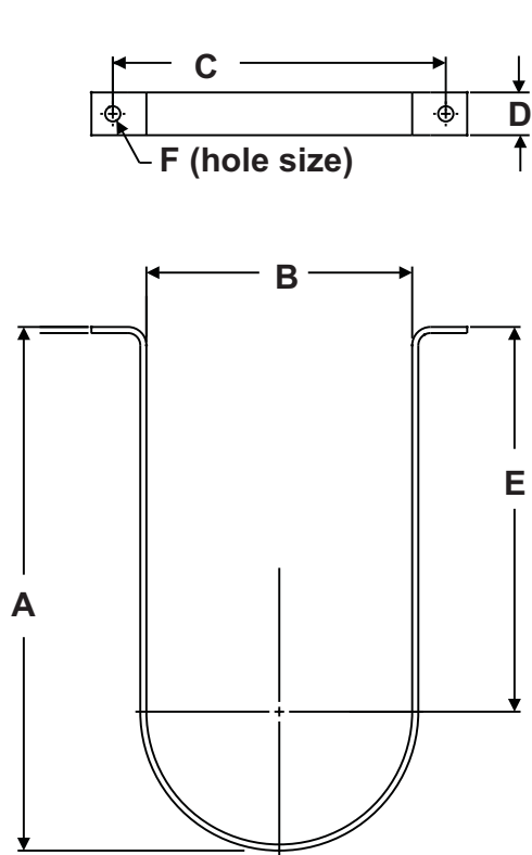
Figure 1. 4070-cu. in. Combined Cylinder Strap (P/N 06-236173-001)
