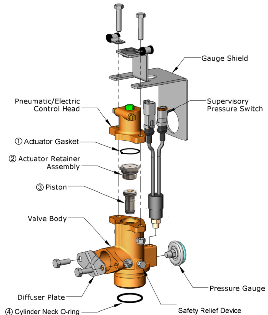
Figure 1. Cylinder Valve Assembly - Exploded View
