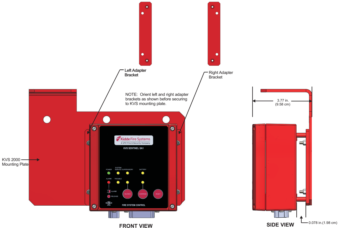
Sentinel SA1 Control Module Mounted Using Adapter Bracket Pair, P/N 83-130034-401
